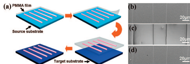
Figure 1. (a) Illustration of the procedures of PMMA-mediated nanotransfer printing technique. Spin-coating a PMMA film on source substrate, peeling off the film from substrate, attaching the film to target substrate, and finally removing the mediator. SEM images of SWNT array (b) on SiO 2 /Si substrate before transfer, (c) embedded in PMMA film, and (d) transferred to another SiO 2 /Si substrate.
