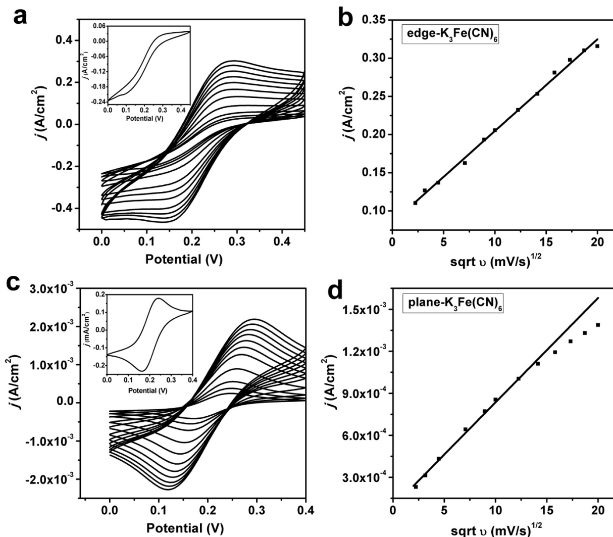
Figure 3 | Electrochemistry of ferricyanide at the graphene edge- or plane-electrode. (a, b) CVs of 5 mM \text{K}_3\text{Fe}(\text{CN})_6 at the graphene edge-electrode at different scan rates (a) and the plot of saturated current density versus square root of scan rate (b); inset of (a) is the CV recorded at 5 \text{ mV s}^{-1} . (c, d) CVs of 5 mM \text{K}_3\text{Fe}(\text{CN})_6 at the graphene plane-electrode at different scan rates (c) and the plot of saturated current density versus square root of scan rate (d); inset of (b) is the CV recorded at 5 \text{ mV s}^{-1} . The electrolyte = 0.1 M PBS + 0.1 M KCl.
